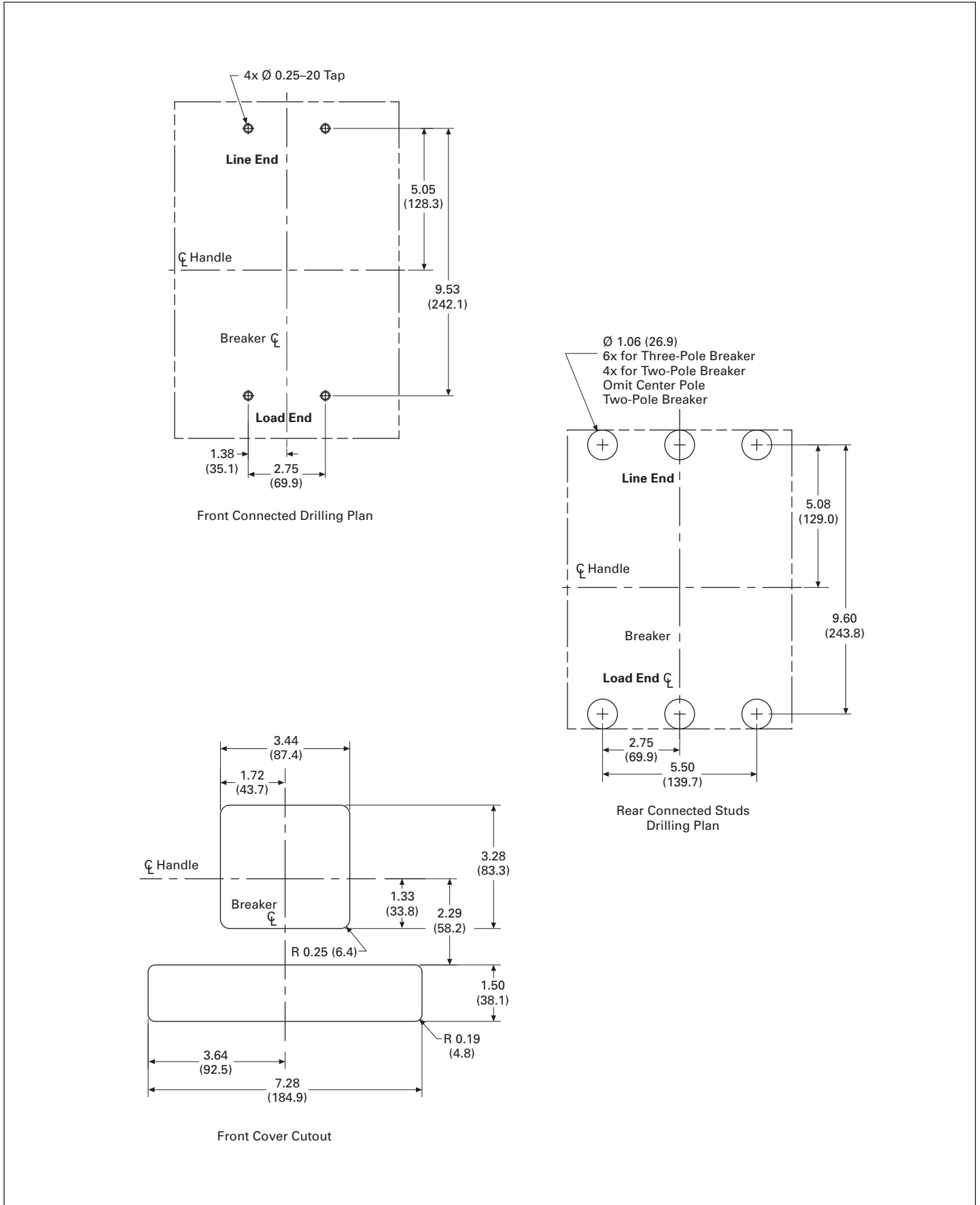
Figure 8. Type LG 450-600A Three-Pole Cutout and Drilling Plan—Dimensions in Inches (mm)
