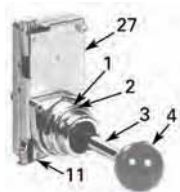
Four-Position Joystick Operator (without Latch)
